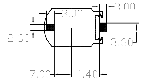
PCB BOARD LAYOUT
