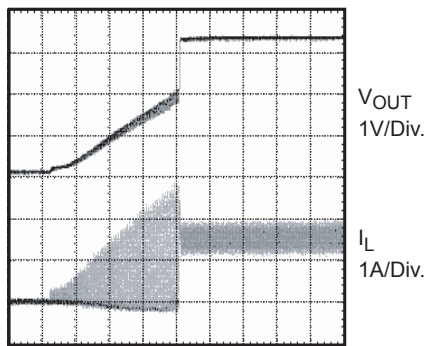
Soft-Start Waveforms
