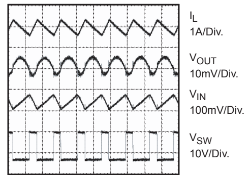
Switching Waveforms
