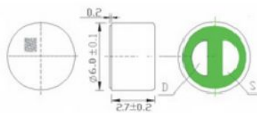
尺寸简图 Dimensions Drawing (Unit: mm)
