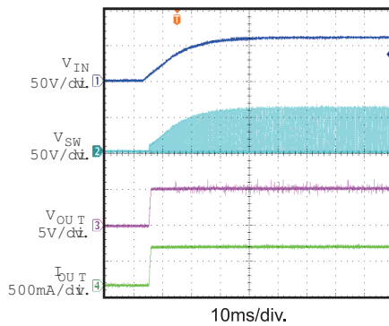
Power Ramp Up V_{IN}=60V , I_{OUT}=0.2A
